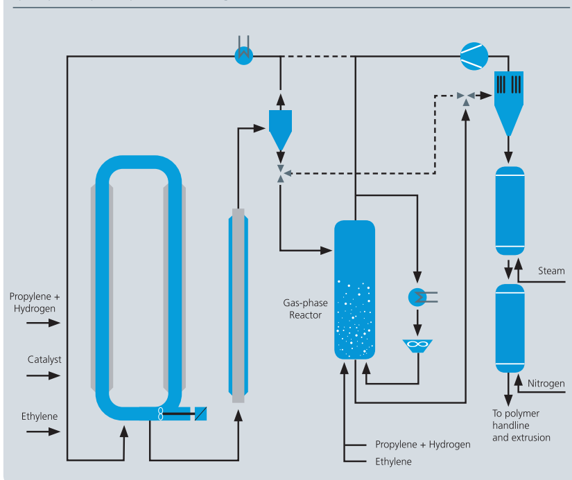
Spheripol simplified process flow diagram
